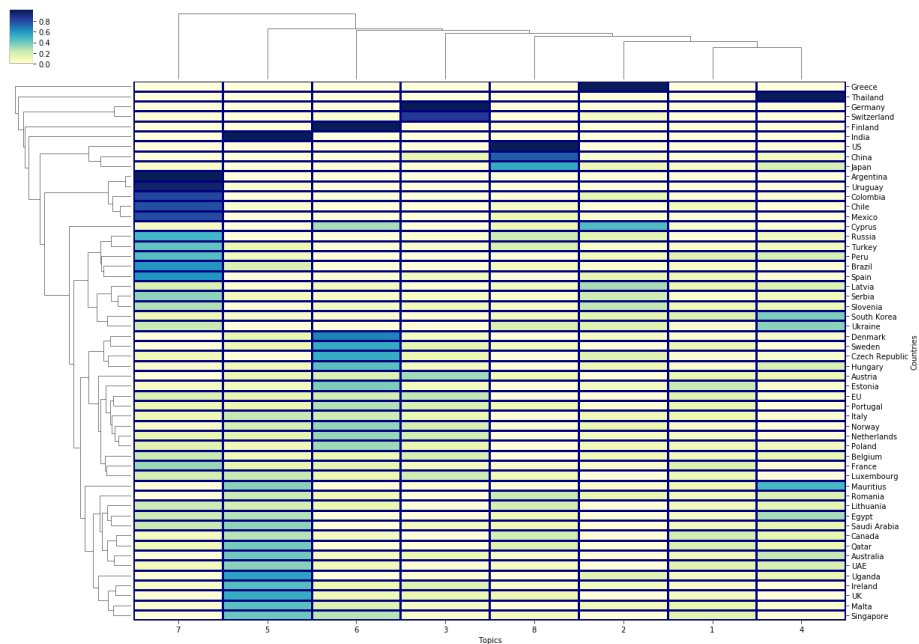
Figure 3: National AI Infrastructures: The heat-map relates per-document/country topic distributions. A blue-to-yellow color-coding scheme indicates high-to-low topic probabilities. The dendrogram at the top shows how topics relate to one another (via the Hellinger distance computed over the word distributions in topics) and cluster via agglomerative hierarchical clustering. The dendrogram at the left shows how countries relate to one another (via the Hellinger distance computed over the topic distributions in documents/countries) and cluster via agglomerative hierarchical clustering.
