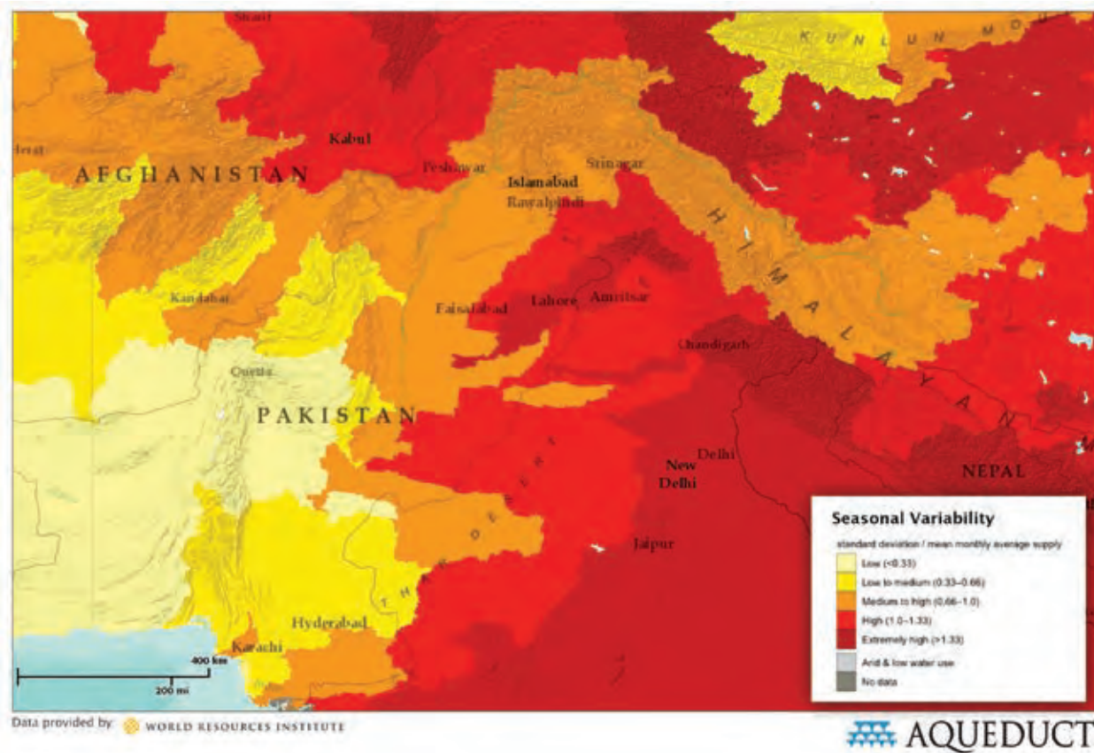
Figure 6. Seasonal Variability of Water Supply in the Indus River Basin
